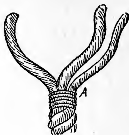
FIG. 105.—Ending rope.
